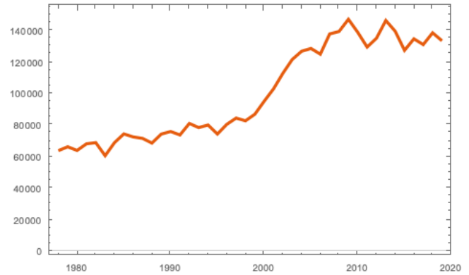
Figure 2: Agricultural productivity in the US.
